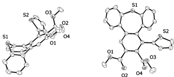
Figure 2. ORTEP diagram of 3ga . Thermal ellipsoids shown at 50% probability. [20]
